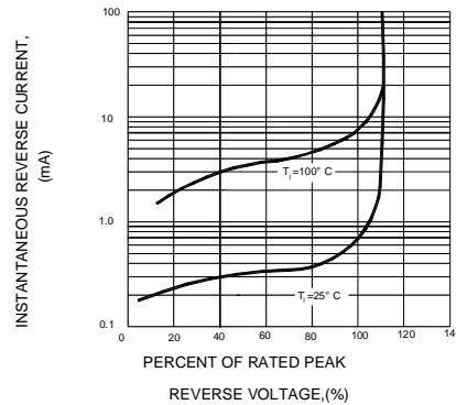
FIG.4-TYPICAL REVERSE CHARACTERISTICS
